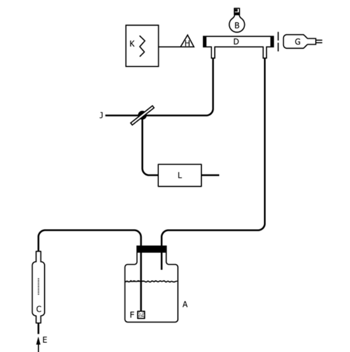
A—Reaction flask B—60-W light bulb C—Rotameter, 1 L of air per minute D—Absorption cell with quartz windows E—Compressed air, 1 L of air per minute F—Glass tube with fritted end G—Hollow cathode mercury lamp H—Atomic absorption detector J—Vent to hood K—Recorder, any compatible model L—To vacuum through gas washing bottle containing 0.25 % iodine in a 3 % potassium iodide solution
